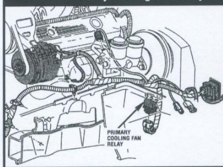
1986-87 Primary Cooling Fan Relay
