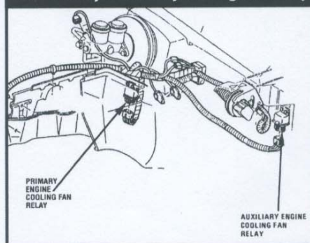
1985 Primary & Auxiliary Cooling Fan Relay
